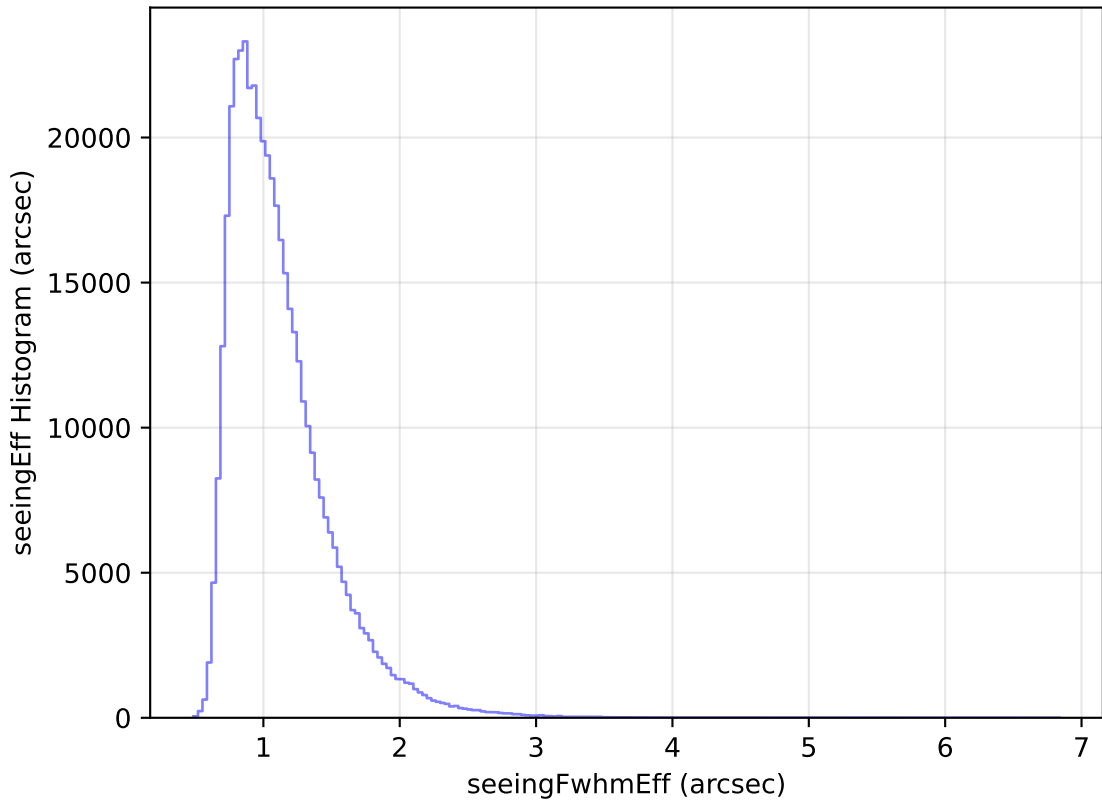
internal_u_expt60_nscale1.0v3.4_10yrs WFD r band: seeingEff Histogram
