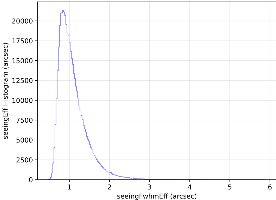
internal_u_expt60_nscale1.0v3.4_10yrs WFD i band: seeingEff Histogram
