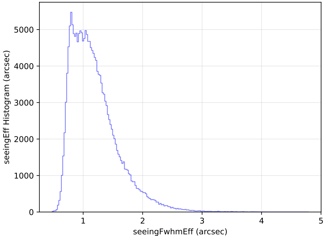
internal_u_expt60_nscale1.0v3.4_10yrs WFD g band: seeingEff Histogram
