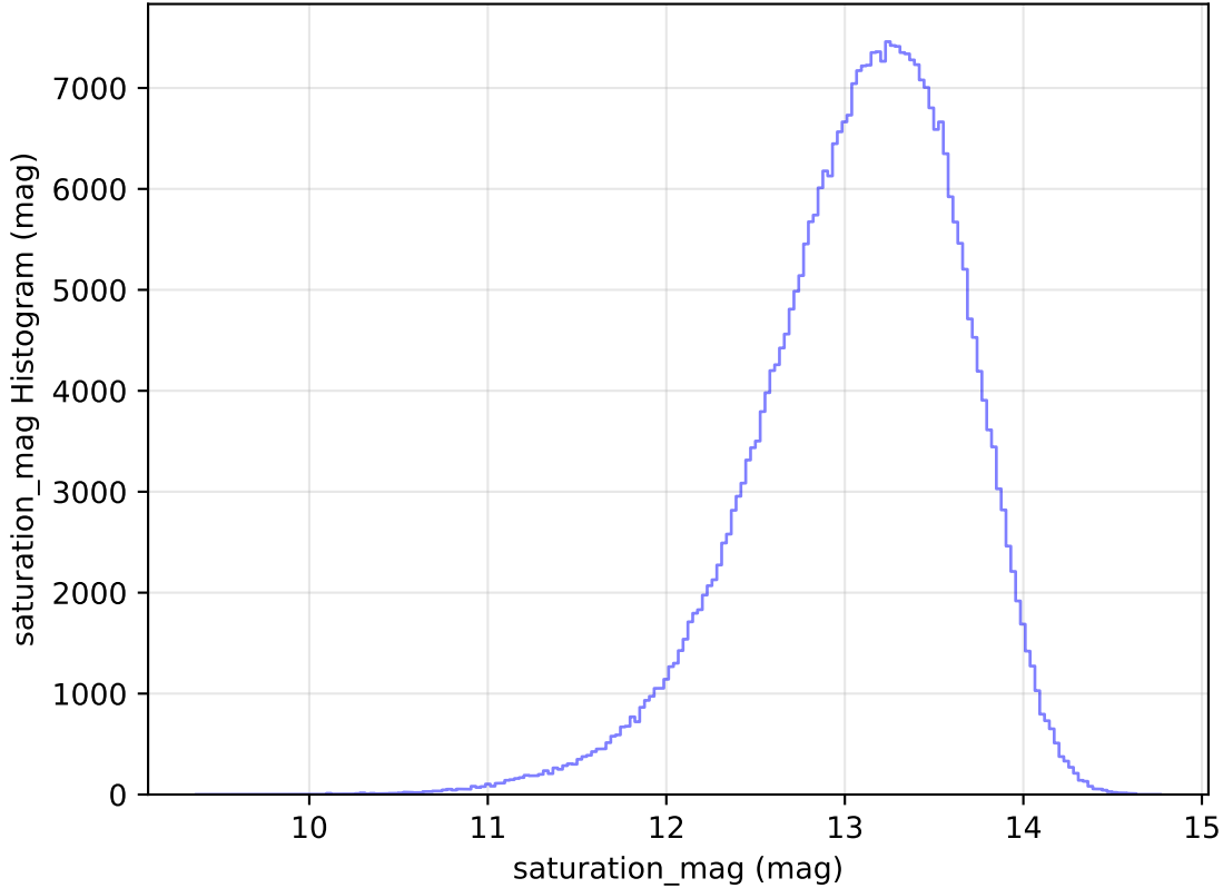
internal_u_expt60_nscale1.0v3.4_10yrs WFD y band: saturation_mag Histogram
