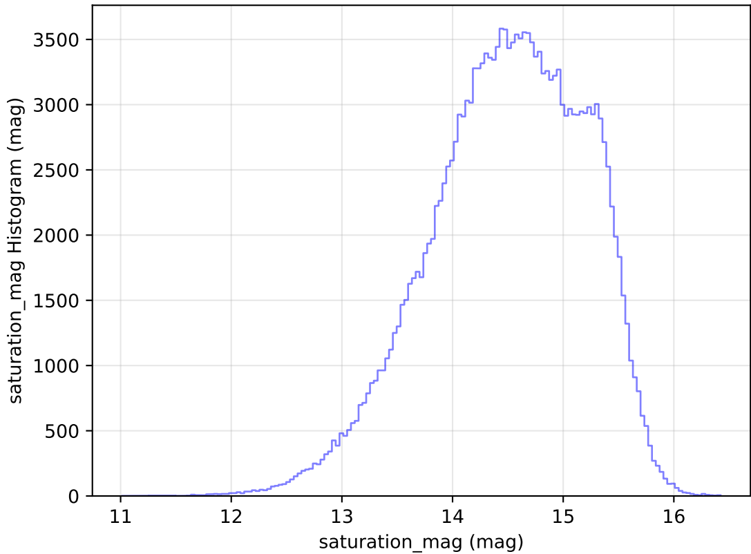
internal_u_expt60_nscale1.0v3.4_10yrs WFD g band: saturation_mag Histogram
