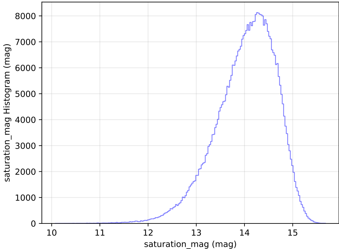
internal_u_expt60_nscale1.0v3.4_10yrs All sky z band: saturation_mag Histogram
