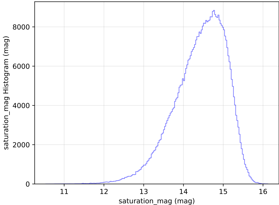
internal_u_expt60_nscale1.0v3.4_10yrs All sky i band: saturation_mag Histogram
