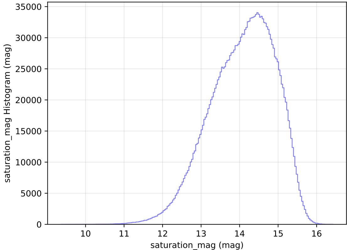
internal_u_expt60_nscale1.0v3.4_10yrs All sky all bands: saturation_mag Histogram
