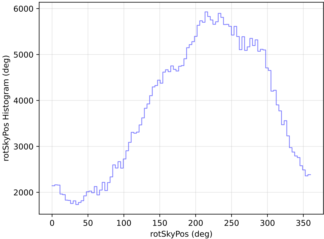
internal_u_expt60_nscale1.0v3.4_10yrs WFD y band: rotSkyPos Histogram
