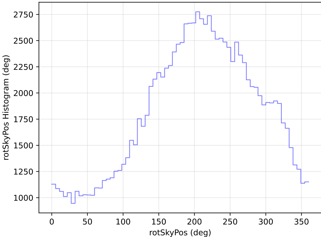
internal_u_expt60_nscale1.0v3.4_10yrs WFD u band: rotSkyPos Histogram
