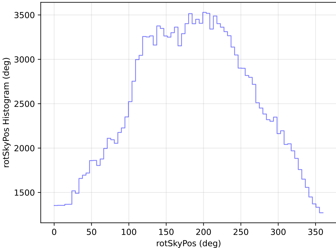
internal_u_expt60_nscale1.0v3.4_10yrs WFD g band: rotSkyPos Histogram
