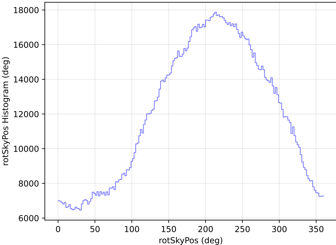
internal_u_expt60_nscale1.0v3.4_10yrs WFD all bands: rotSkyPos Histogram
