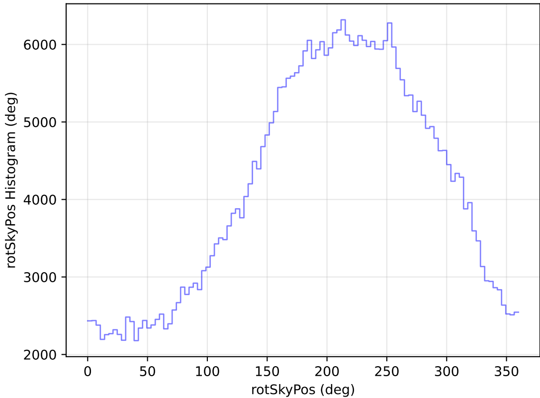
internal_u_expt60_nscale1.0v3.4_10yrs All sky z band: rotSkyPos Histogram
