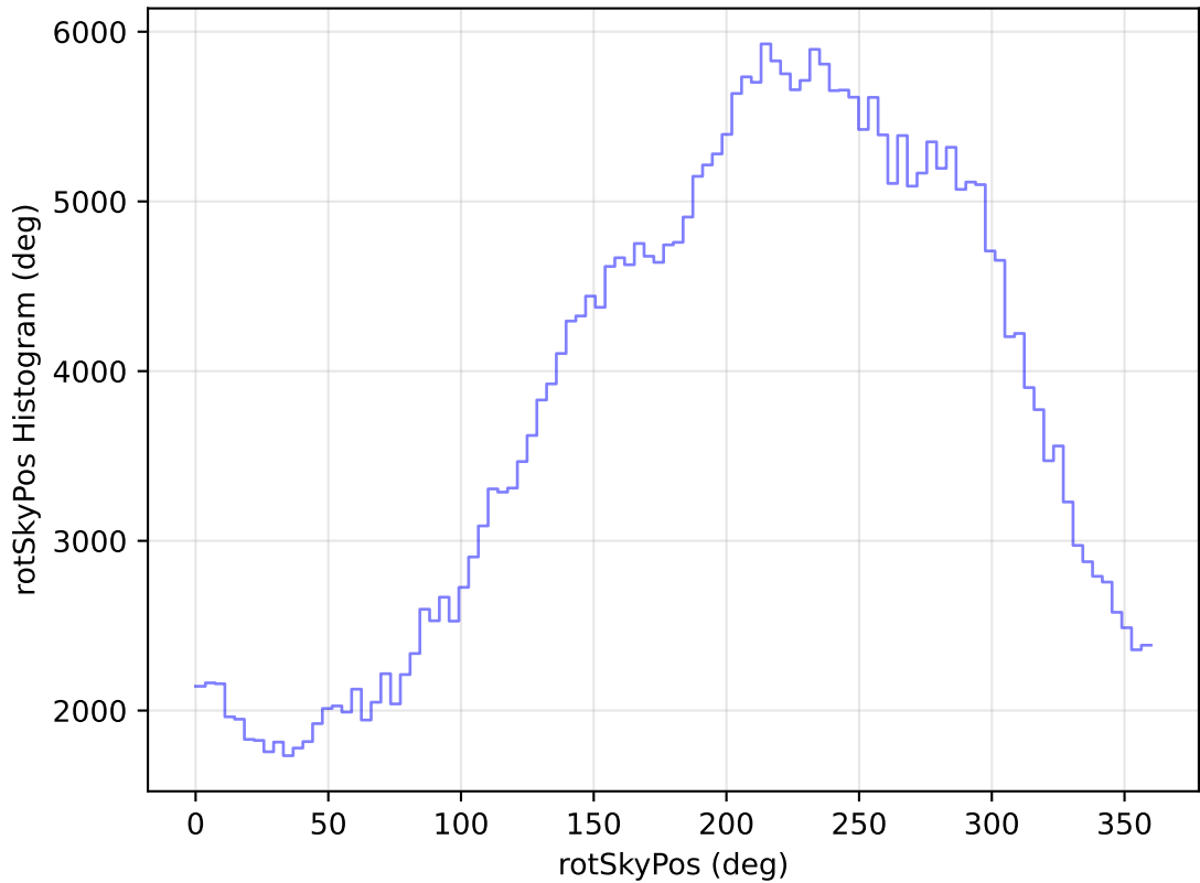
internal_u_expt60_nscale1.0v3.4_10yrs All sky y band: rotSkyPos Histogram
