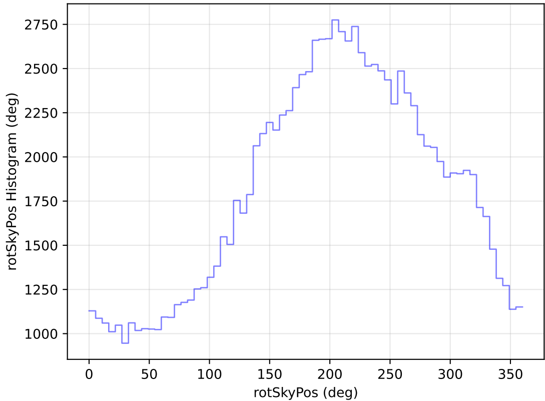
internal_u_expt60_nscale1.0v3.4_10yrs All sky u band: rotSkyPos Histogram
