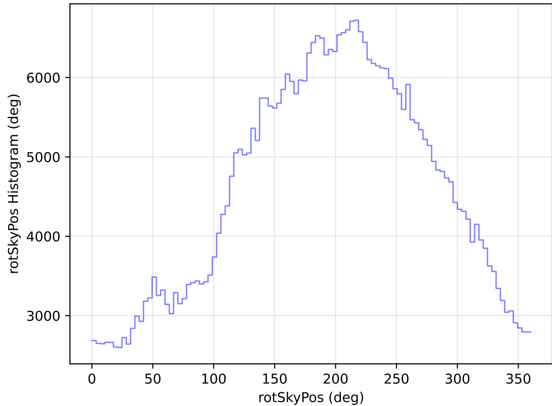
internal_u_expt60_nscale1.0v3.4_10yrs All sky r band: rotSkyPos Histogram
