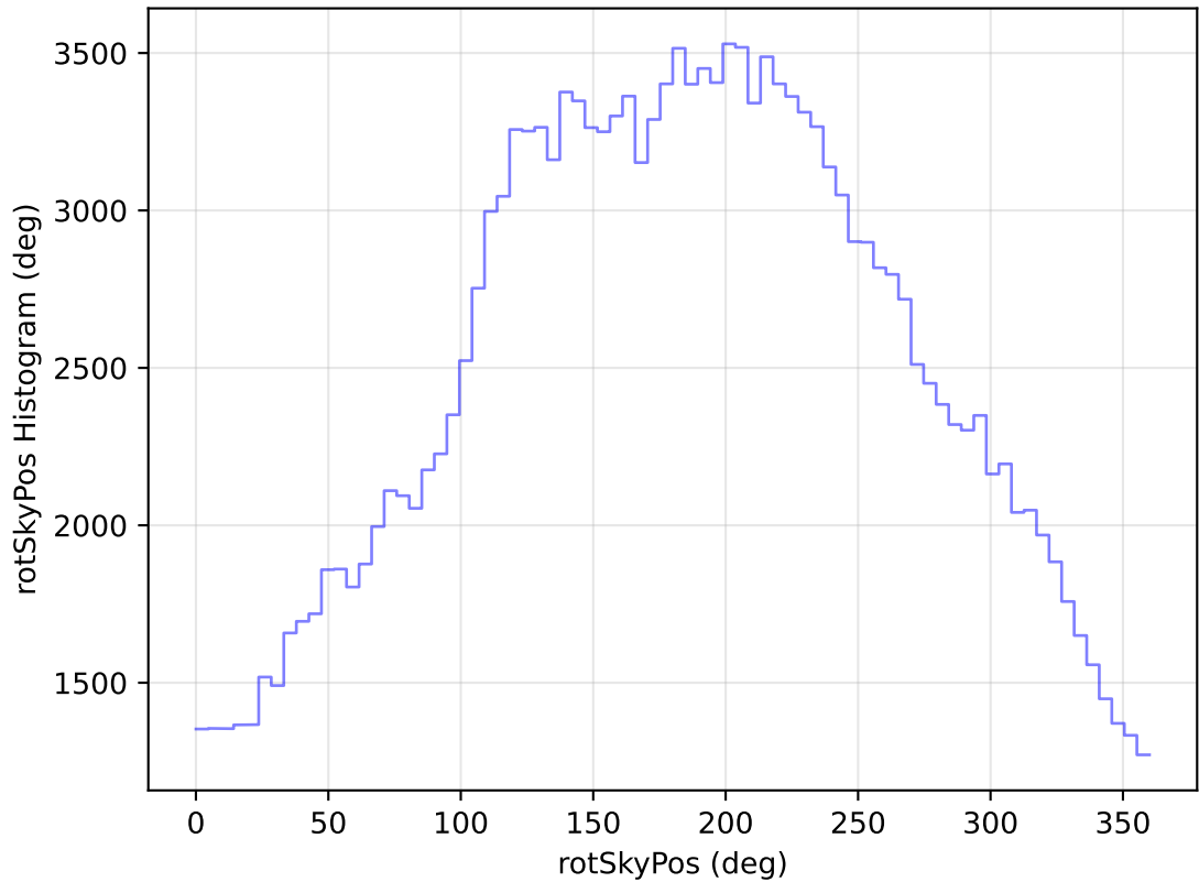
internal_u_expt60_nscale1.0v3.4_10yrs All sky g band: rotSkyPos Histogram
