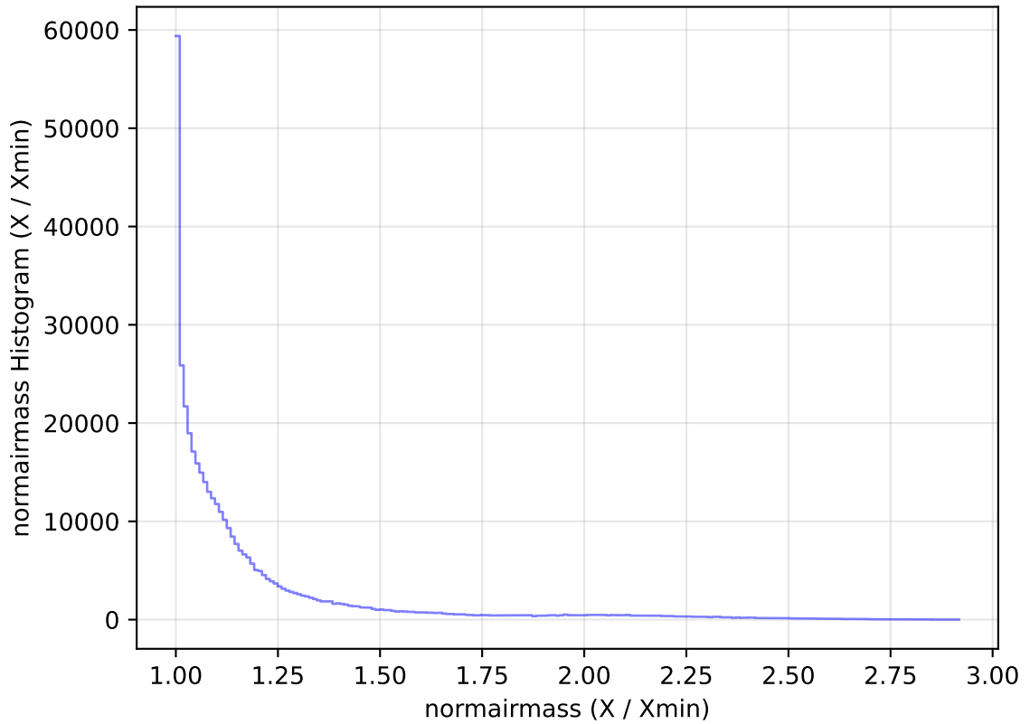
internal_u_expt60_nscale1.0v3.4_10yrs WFD z band: normairmass Histogram
