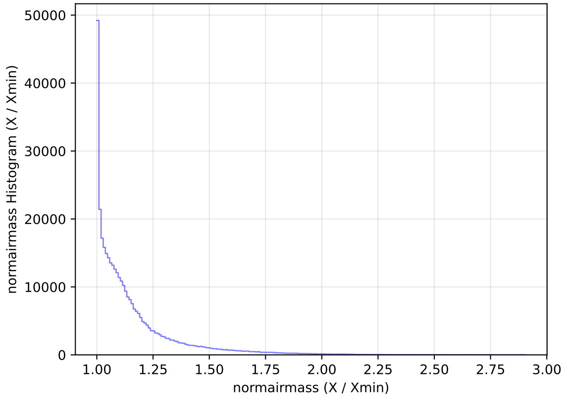
internal_u_expt60_nscale1.0v3.4_10yrs WFD y band: normairmass Histogram
