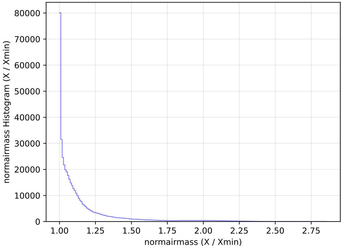
internal_u_expt60_nscale1.0v3.4_10yrs WFD r band: normairmass Histogram
