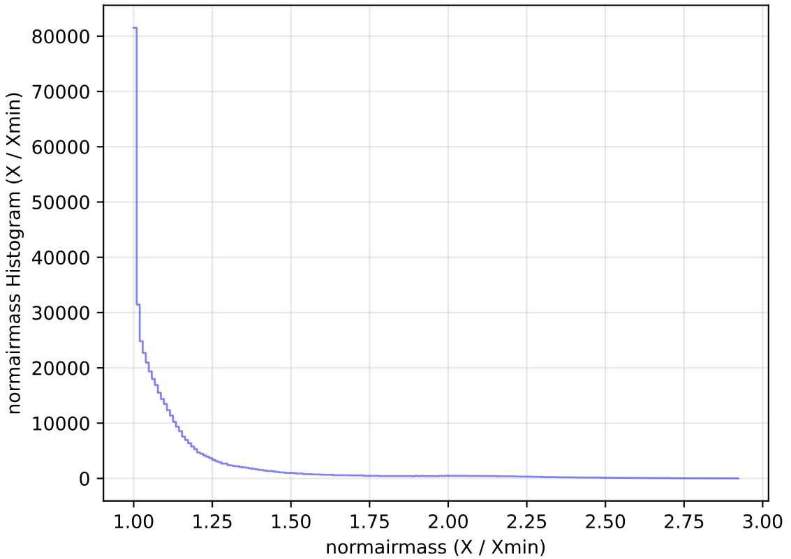
internal_u_expt60_nscale1.0v3.4_10yrs WFD i band: normairmass Histogram
