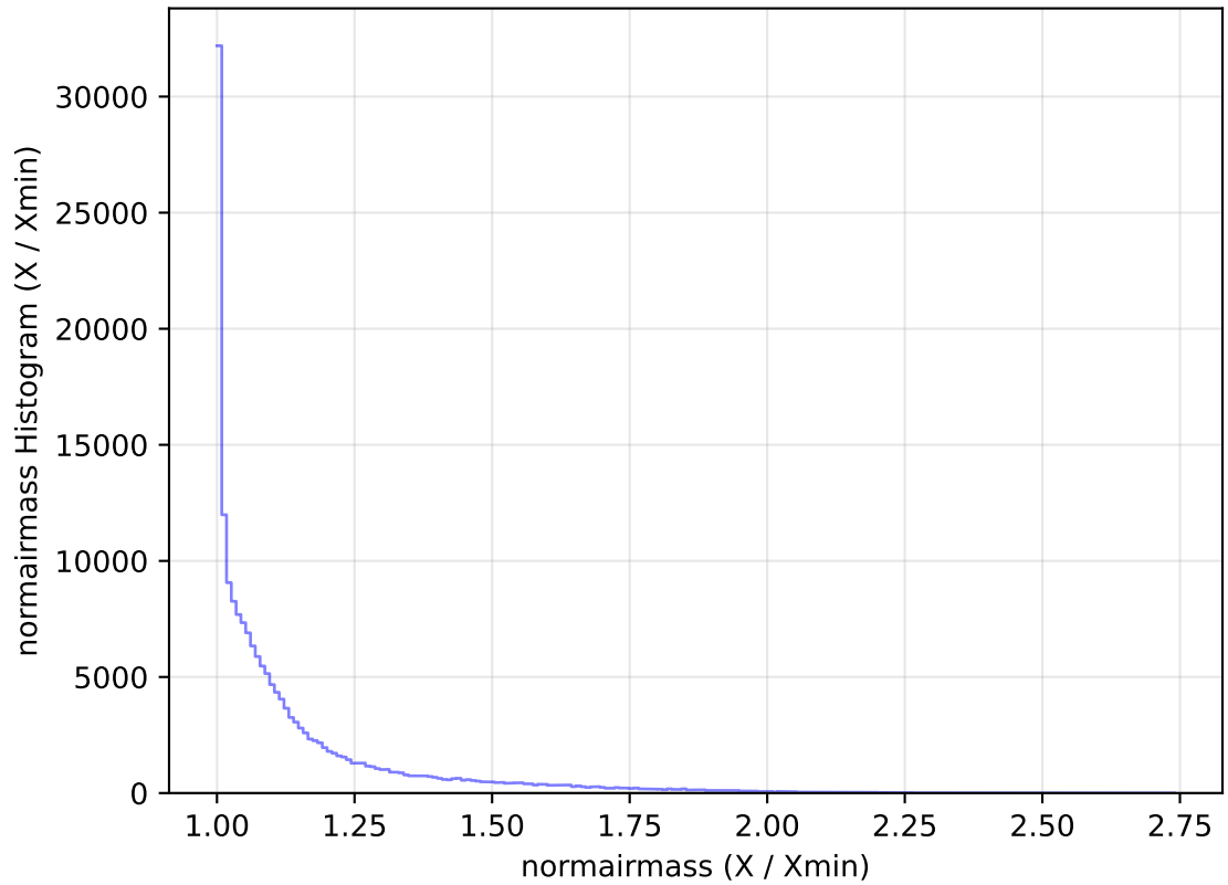
internal_u_expt60_nscale1.0v3.4_10yrs WFD g band: normairmass Histogram
