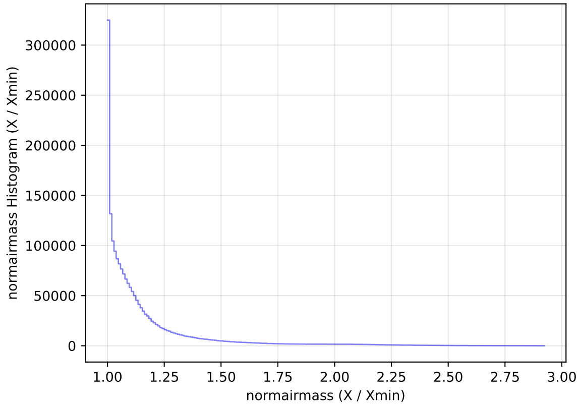
internal_u_expt60_nscale1.0v3.4_10yrs WFD all bands: normairmass Histogram
