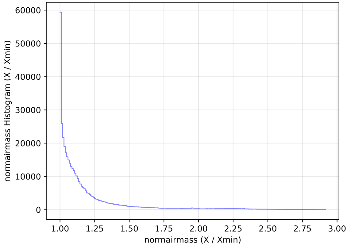
internal_u_expt60_nscale1.0v3.4_10yrs All sky z band: normairmass Histogram
