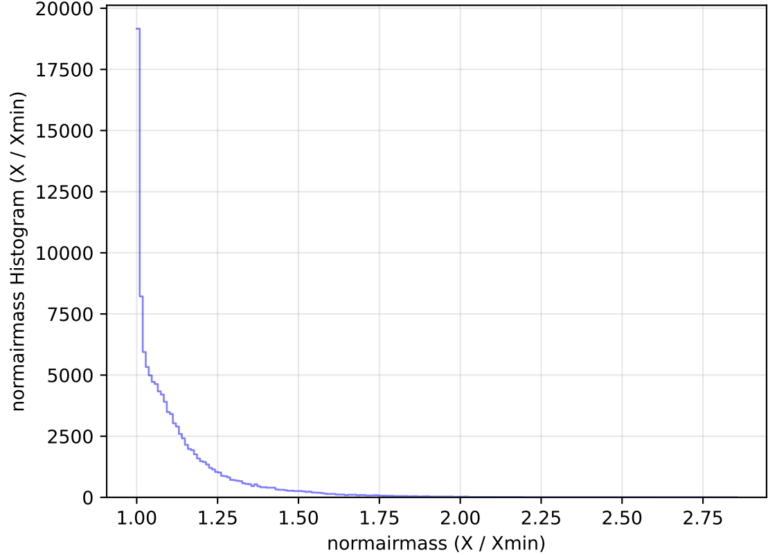
internal_u_expt60_nscale1.0v3.4_10yrs All sky u band: normairmass Histogram
