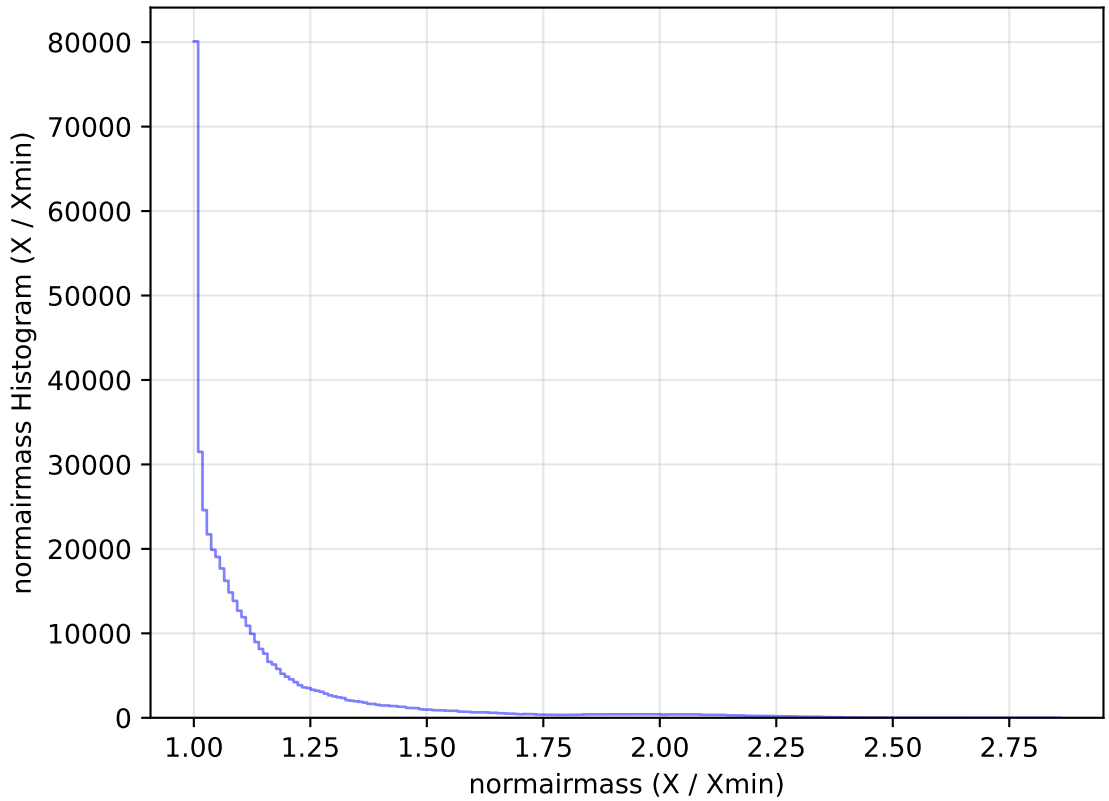
internal_u_expt60_nscale1.0v3.4_10yrs All sky r band: normairmass Histogram
