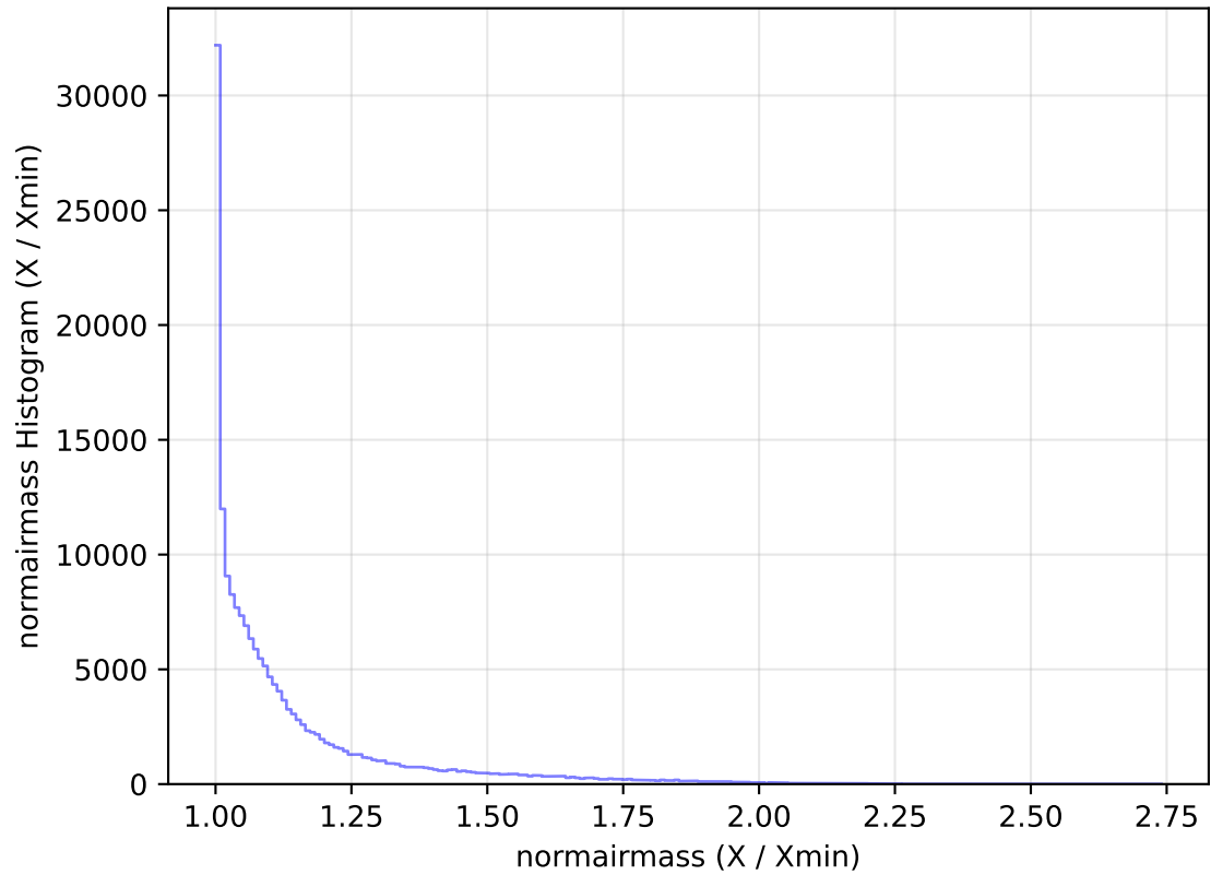
internal_u_expt60_nscale1.0v3.4_10yrs All sky g band: normairmass Histogram
