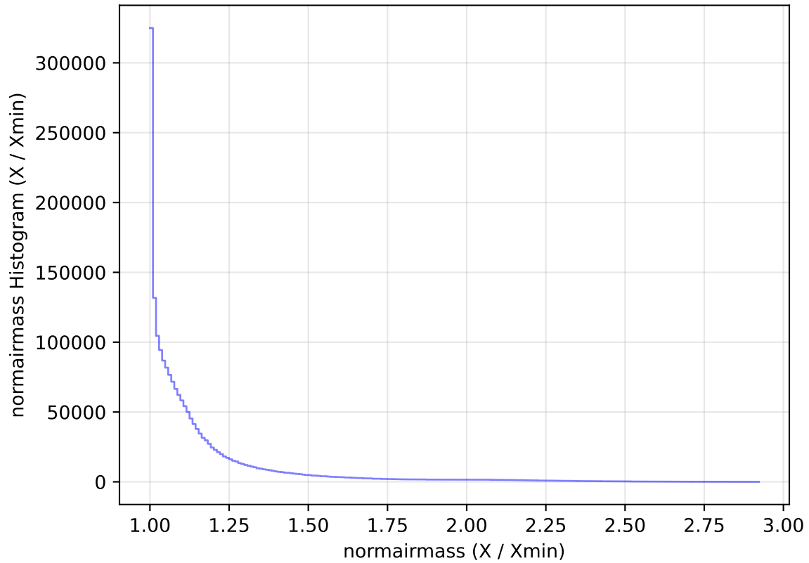
internal_u_expt60_nscale1.0v3.4_10yrs All sky all bands: normairmass Histogram
