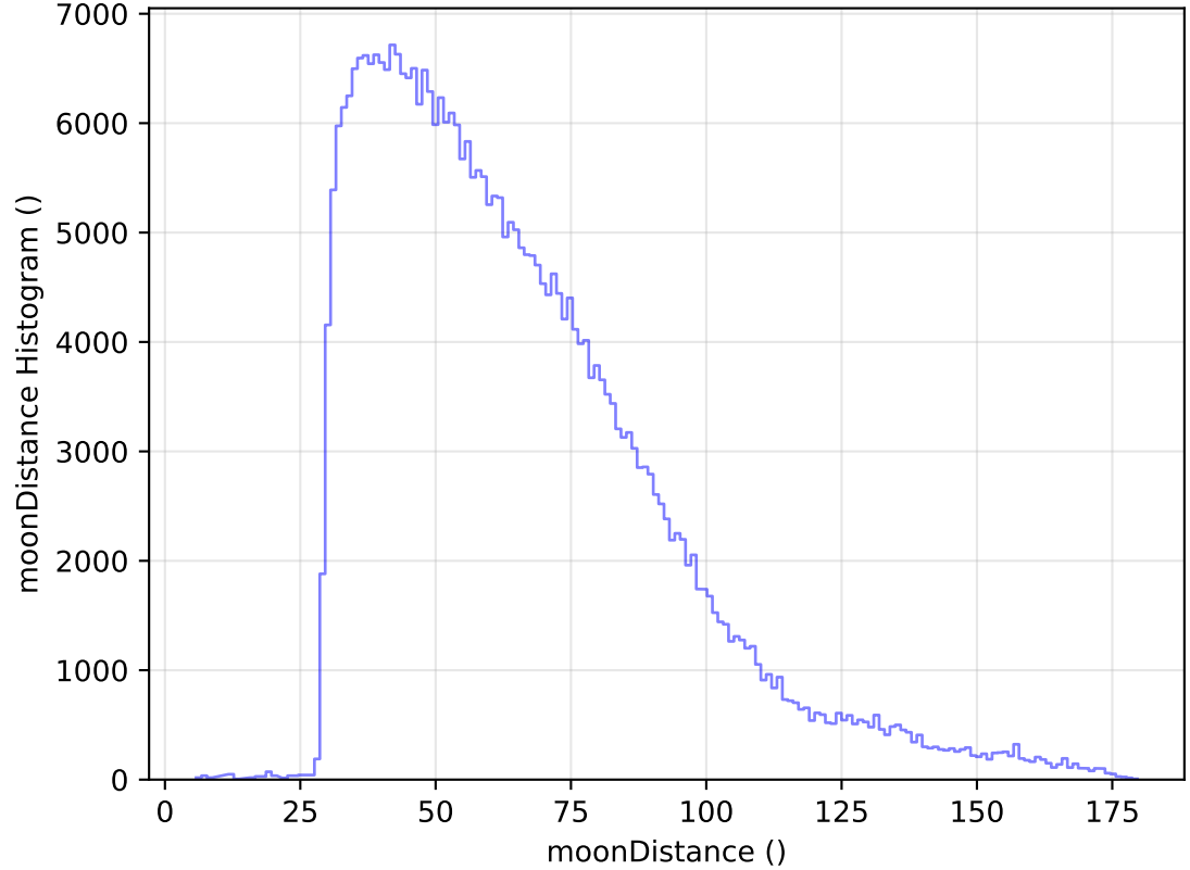
internal_u_expt60_nscale1.0v3.4_10yrs WFD y band: moonDistance Histogram
