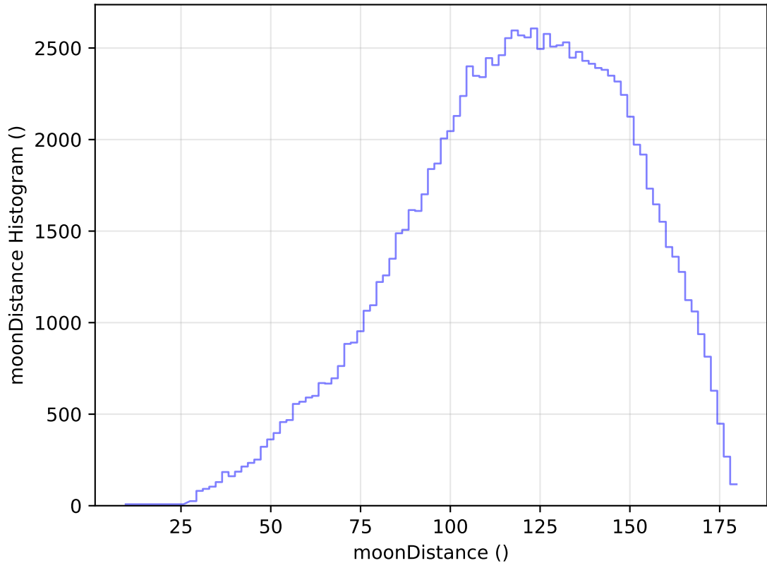
internal_u_expt60_nscale1.0v3.4_10yrs WFD u band: moonDistance Histogram
