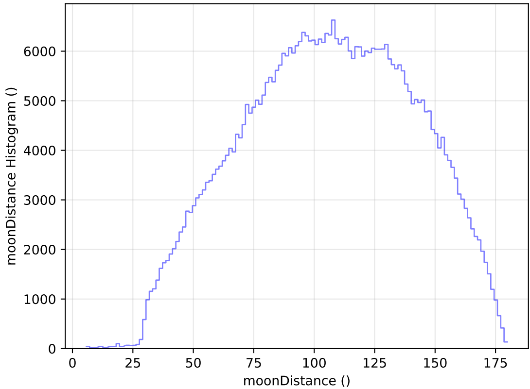
internal_u_expt60_nscale1.0v3.4_10yrs WFD r band: moonDistance Histogram
