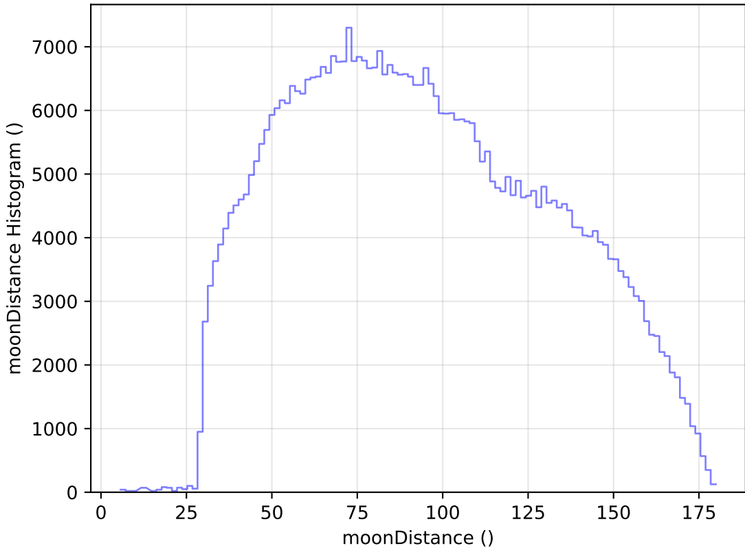
internal_u_expt60_nscale1.0v3.4_10yrs WFD i band: moonDistance Histogram
