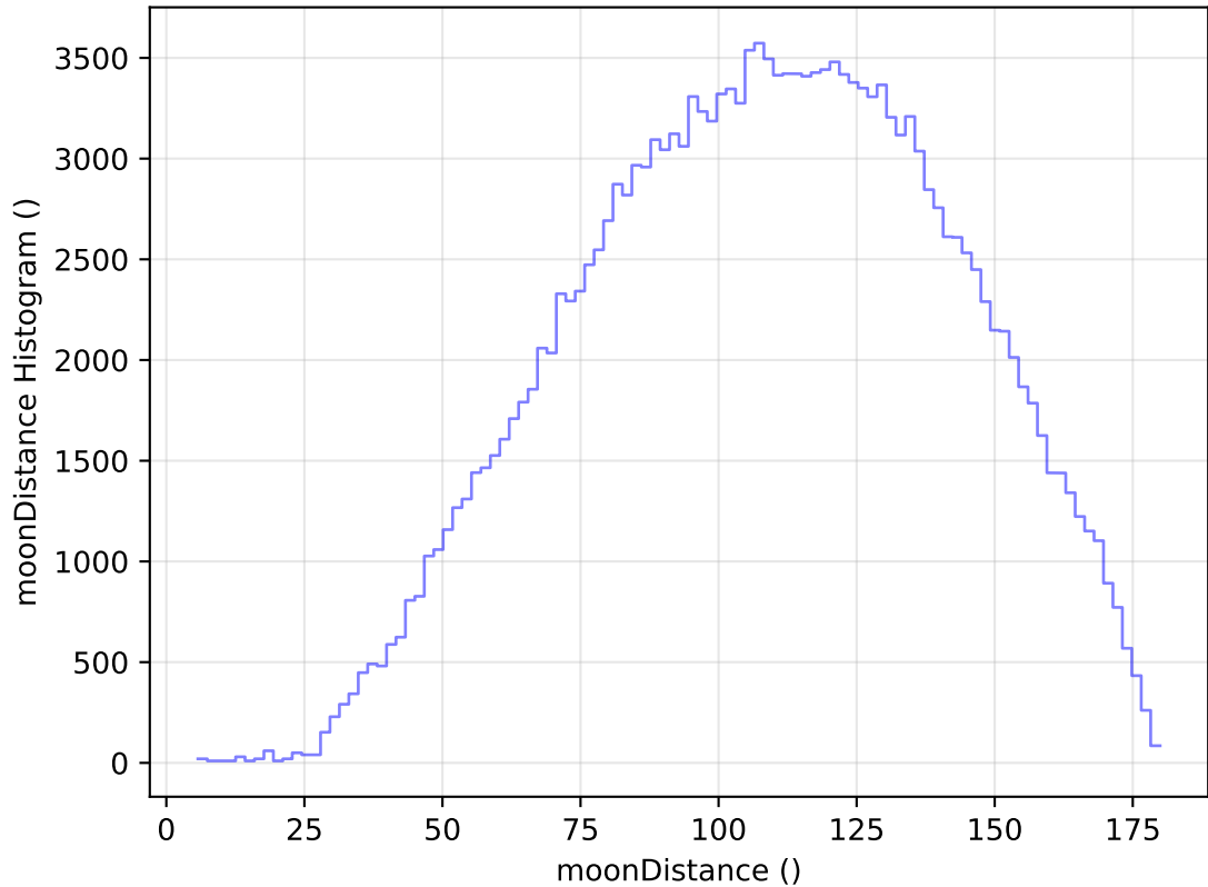
internal_u_expt60_nscale1.0v3.4_10yrs WFD g band: moonDistance Histogram
