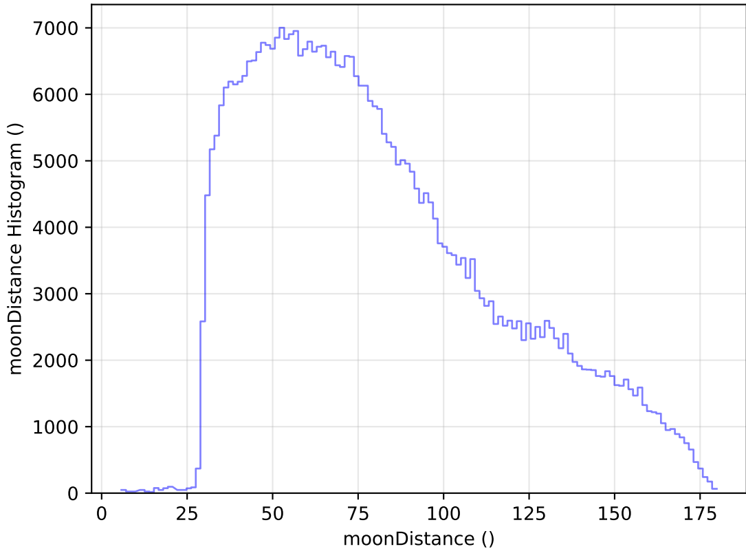
internal_u_expt60_nscale1.0v3.4_10yrs All sky z band: moonDistance Histogram
