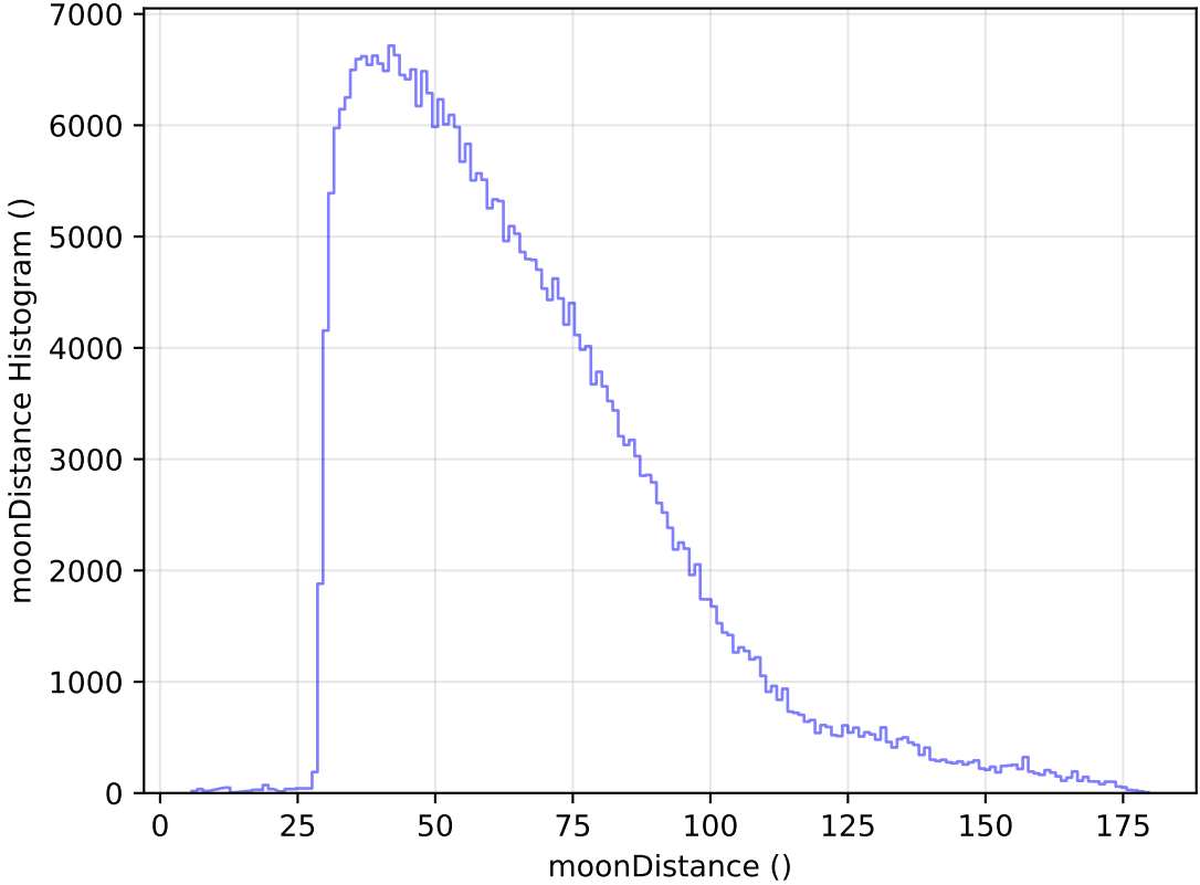
internal_u_expt60_nscale1.0v3.4_10yrs All sky y band: moonDistance Histogram
