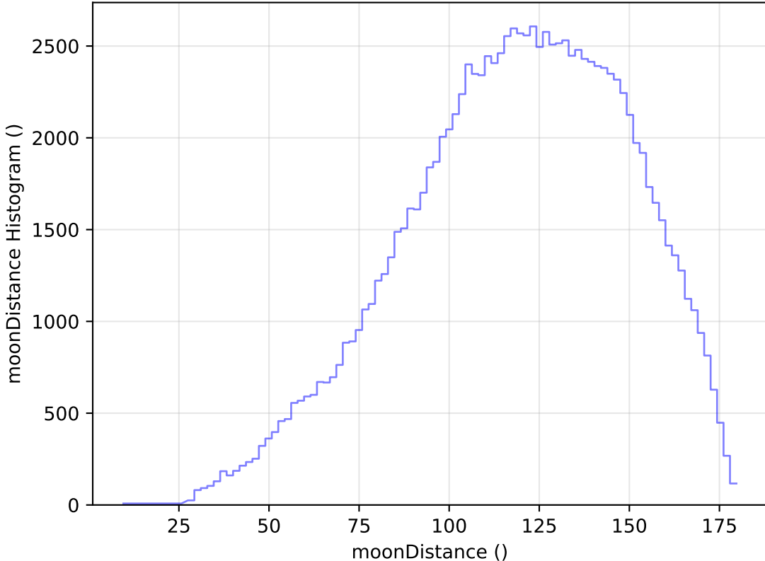
internal_u_expt60_nscale1.0v3.4_10yrs All sky u band: moonDistance Histogram
