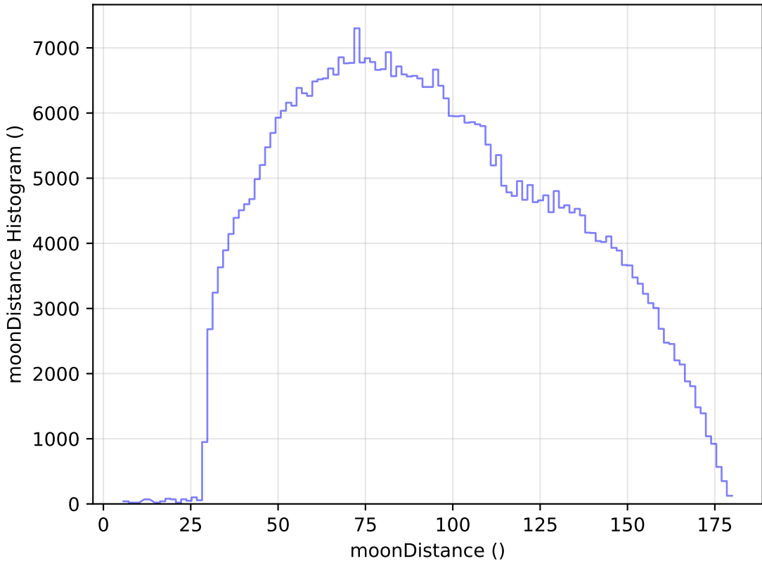
internal_u_expt60_nscale1.0v3.4_10yrs All sky i band: moonDistance Histogram
