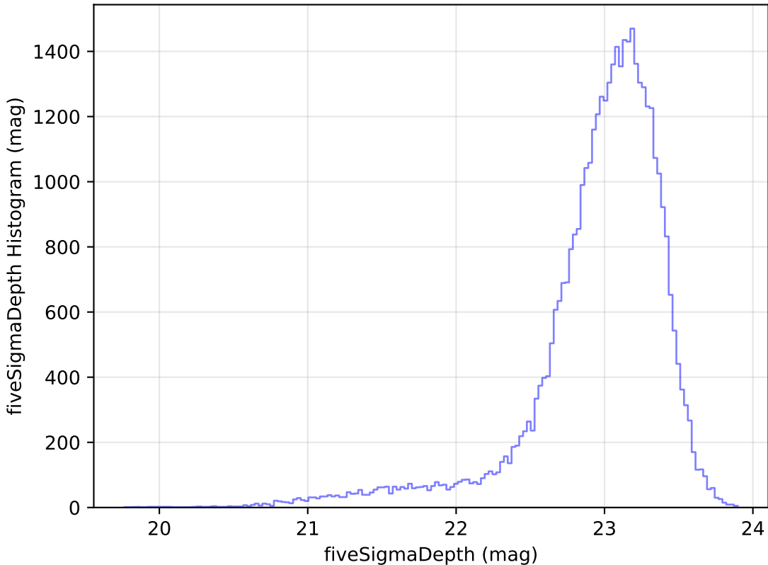
internal_u_expt60_nscale1.0v3.4_10yrs Yr 1 z band: fiveSigmaDepth Histogram
