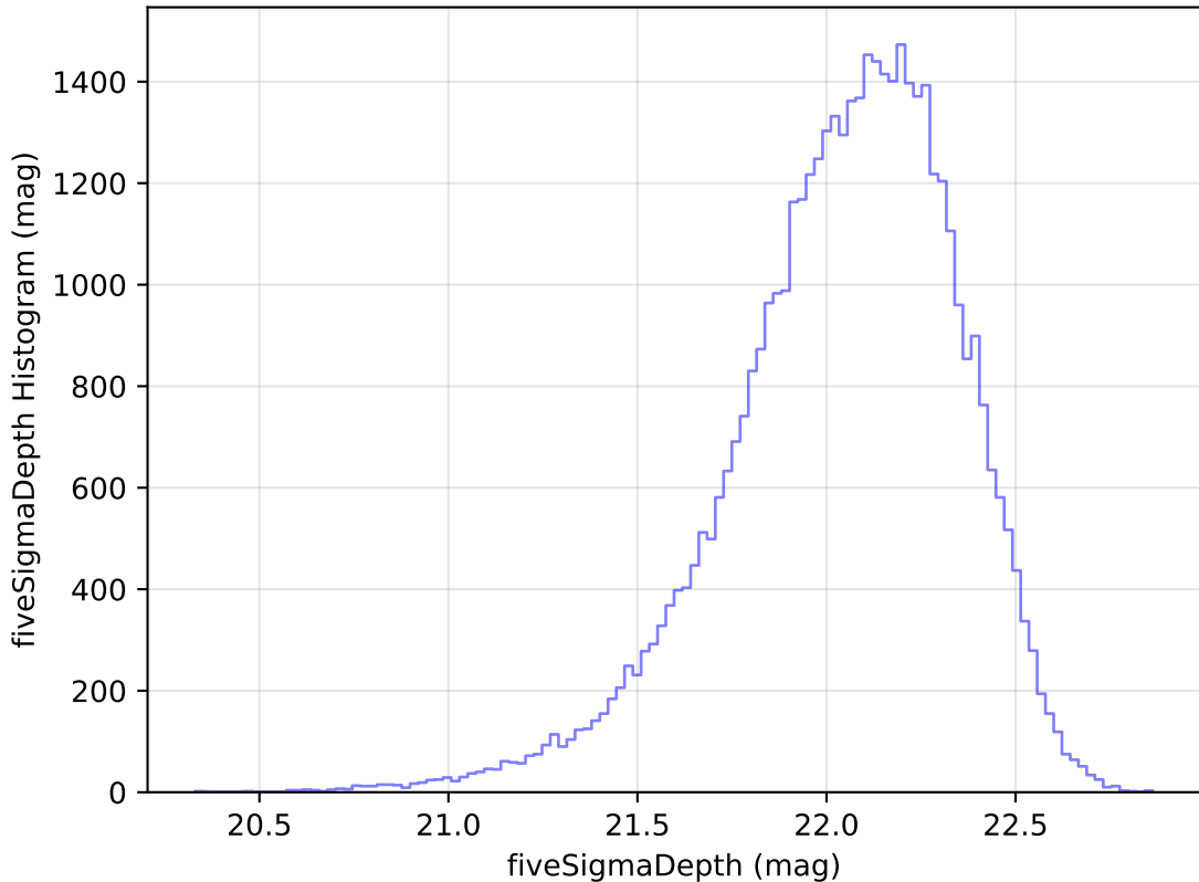
internal_u_expt60_nscale1.0v3.4_10yrs Yr 1 y band: fiveSigmaDepth Histogram
