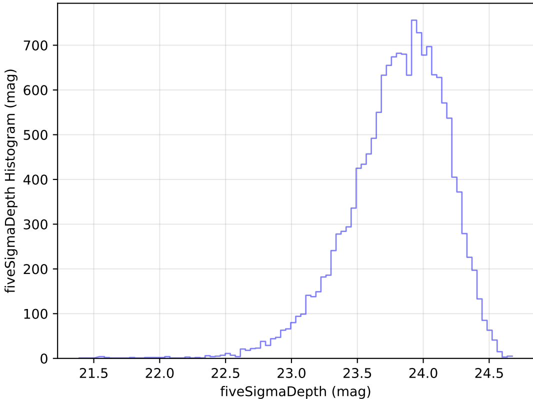
internal_u_expt60_nscale1.0v3.4_10yrs Yr 1 u band: fiveSigmaDepth Histogram
