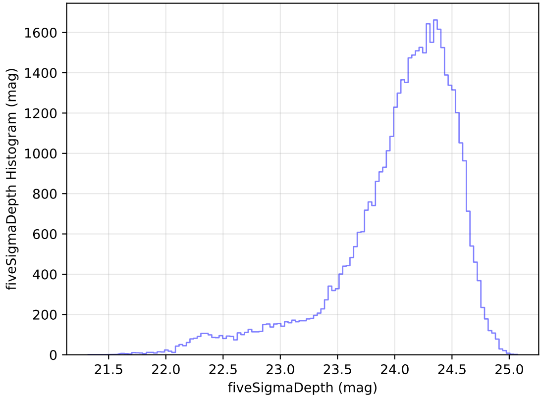
internal_u_expt60_nscale1.0v3.4_10yrs Yr 1 r band: fiveSigmaDepth Histogram
