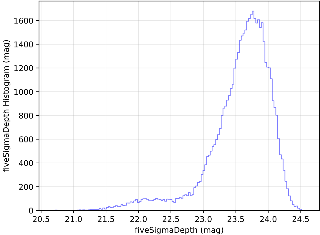
internal_u_expt60_nscale1.0v3.4_10yrs Yr 1 i band: fiveSigmaDepth Histogram
