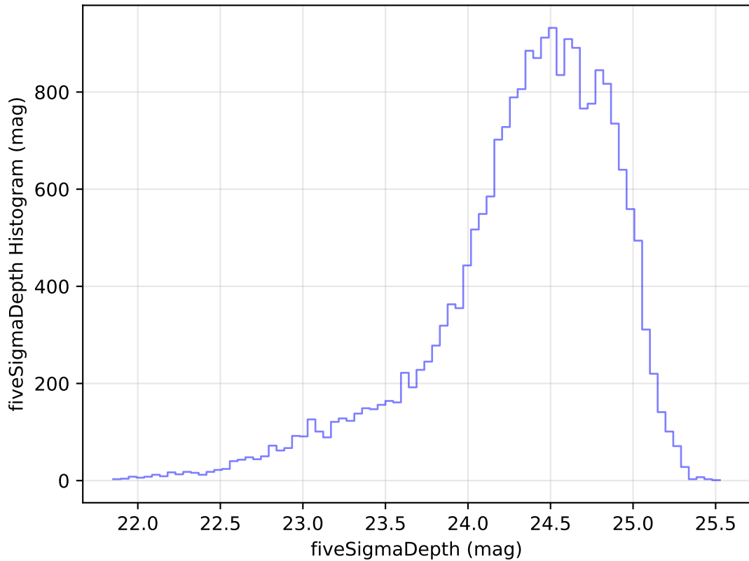
internal_u_expt60_nscale1.0v3.4_10yrs Yr 1 g band: fiveSigmaDepth Histogram
