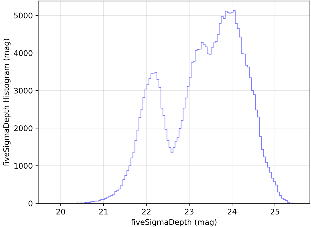
internal_u_expt60_nscale1.0v3.4_10yrs Yr 1 all bands: fiveSigmaDepth Histogram
