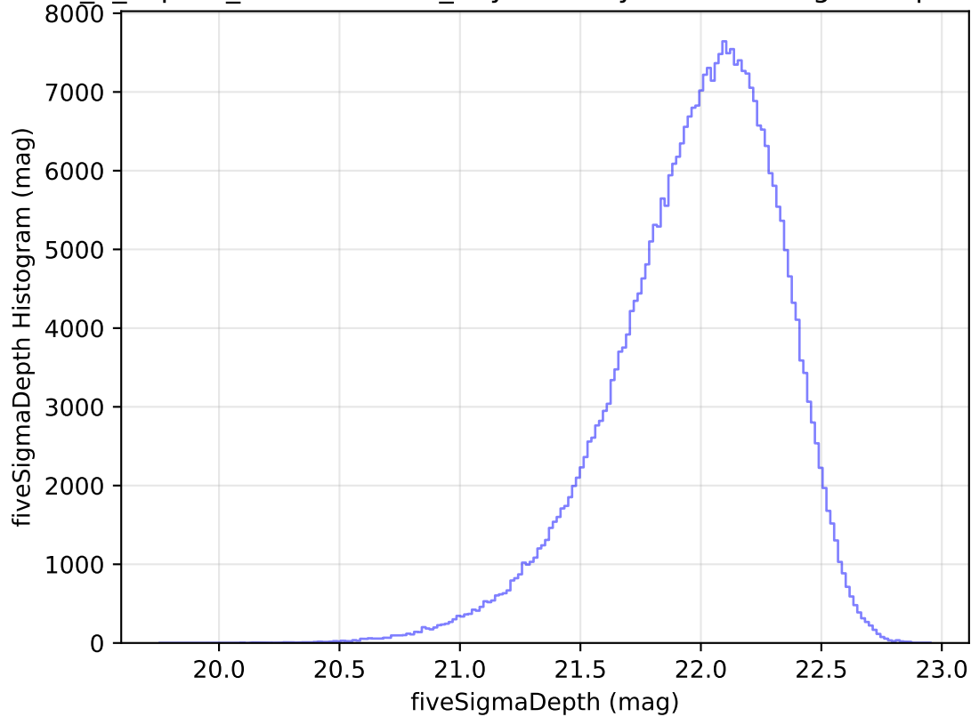
internal_u_expt60_nscale1.0v3.4_10yrs WFD y band: fiveSigmaDepth Histogram
