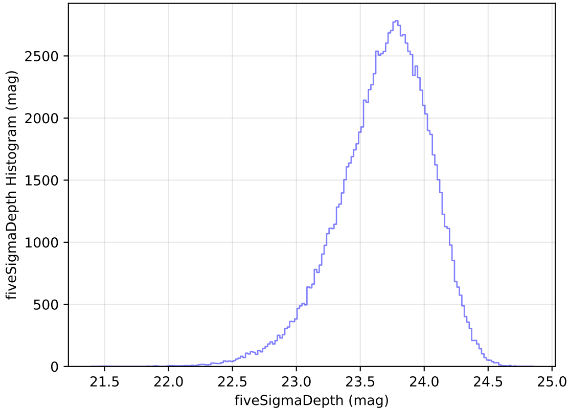
internal_u_expt60_nscale1.0v3.4_10yrs WFD u band: fiveSigmaDepth Histogram
