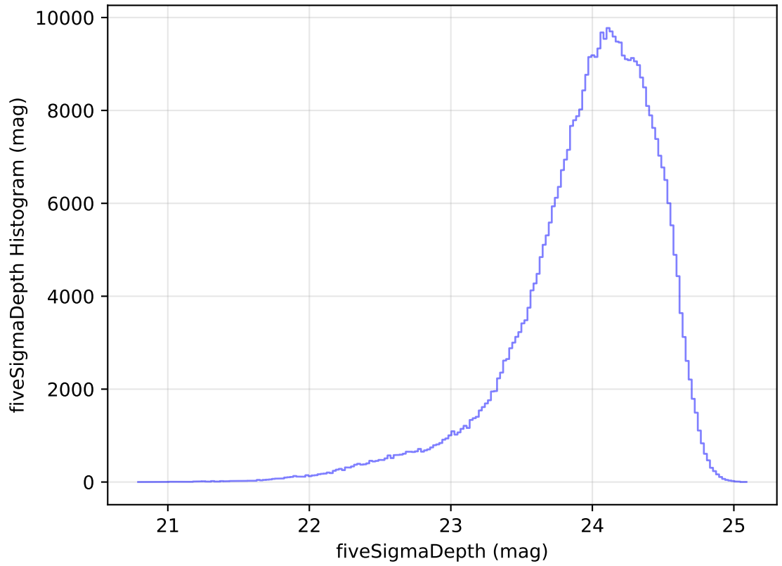
internal_u_expt60_nscale1.0v3.4_10yrs WFD r band: fiveSigmaDepth Histogram
