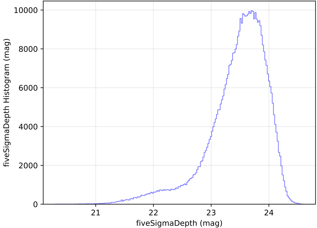
internal_u_expt60_nscale1.0v3.4_10yrs WFD i band: fiveSigmaDepth Histogram
