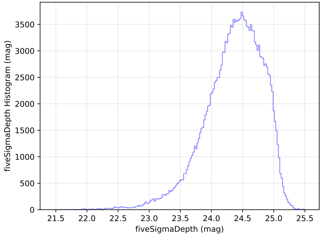
internal_u_expt60_nscale1.0v3.4_10yrs WFD g band: fiveSigmaDepth Histogram
