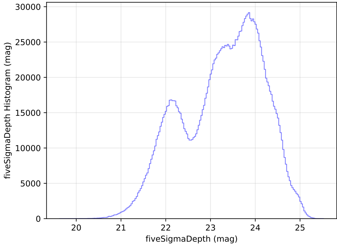
internal_u_expt60_nscale1.0v3.4_10yrs WFD all bands: fiveSigmaDepth Histogram
